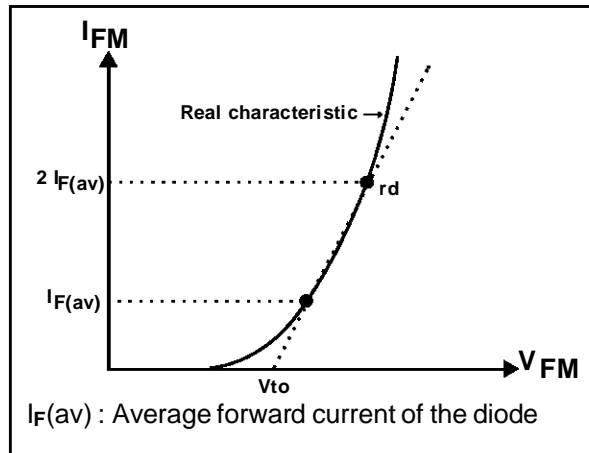
Fig.1 : Forward characteristics of a diodes
